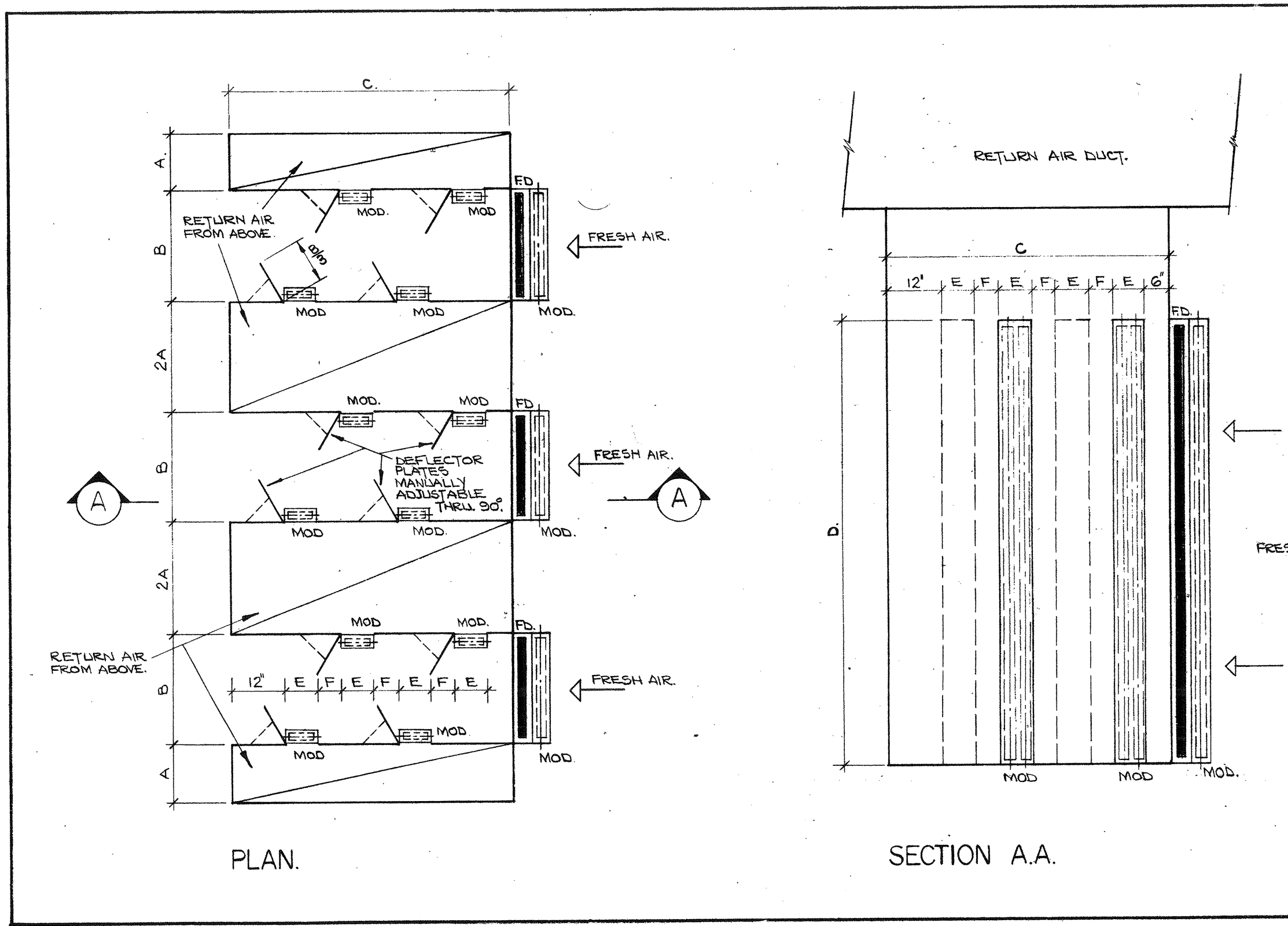
10 DETAIL OF A.C. UNIT AIR MIXING PLENUMS. N.T.S.
