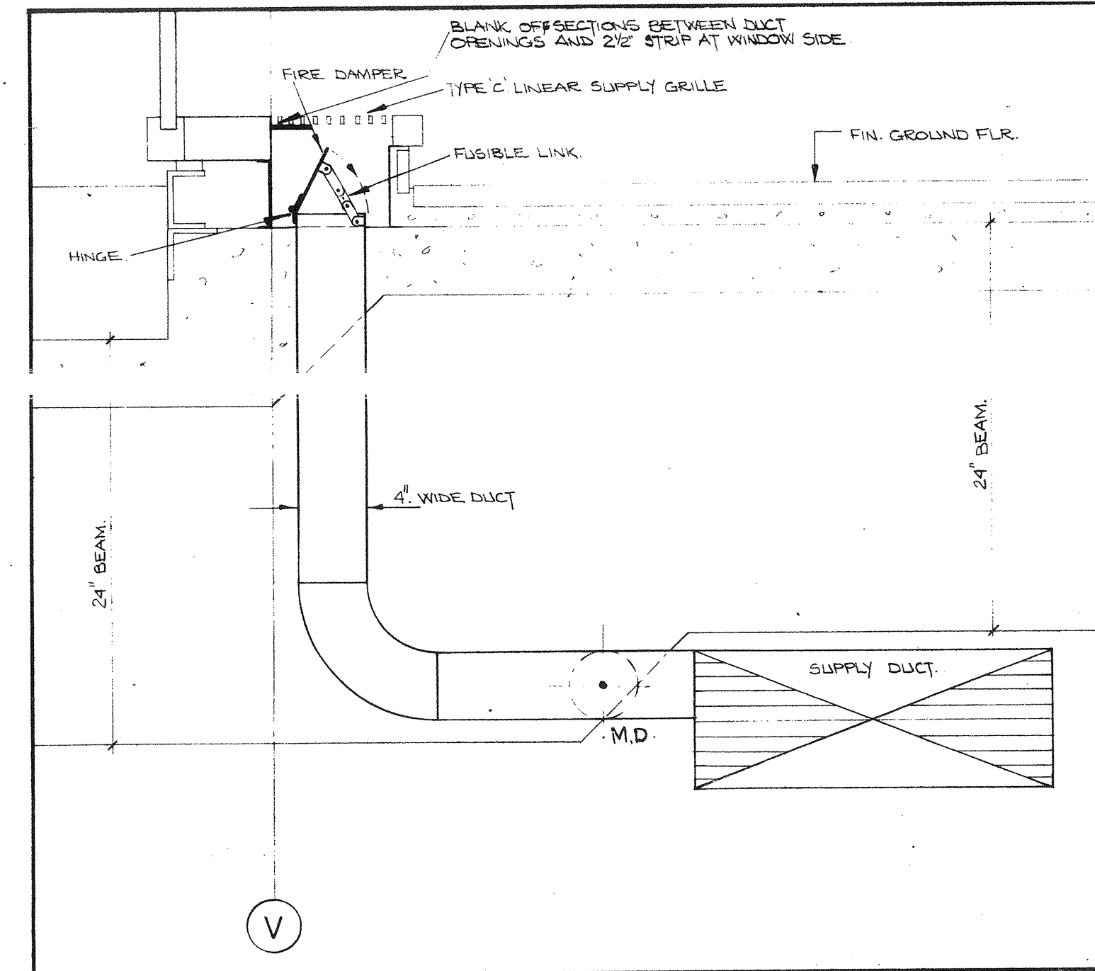
9 GROUND FLOOR EAST WINDOW SUPPLY DETAIL BETWEEN GRID LINES 11 & 33. SCALE: 1 1/2"=1'-0".
