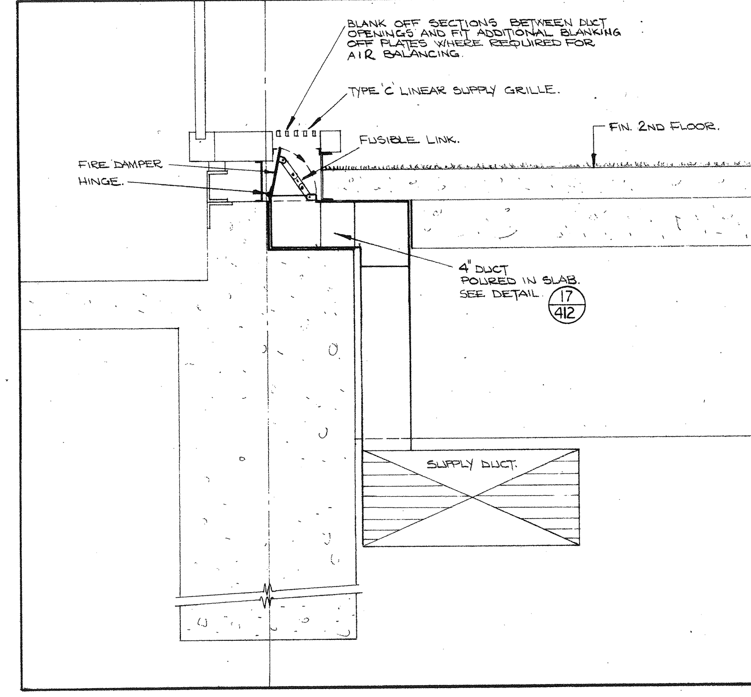
11 TYPICAL SECOND FLOOR WINDOW SUPPLY DETAIL. SCALE: 1 1/2"=1'-0".
