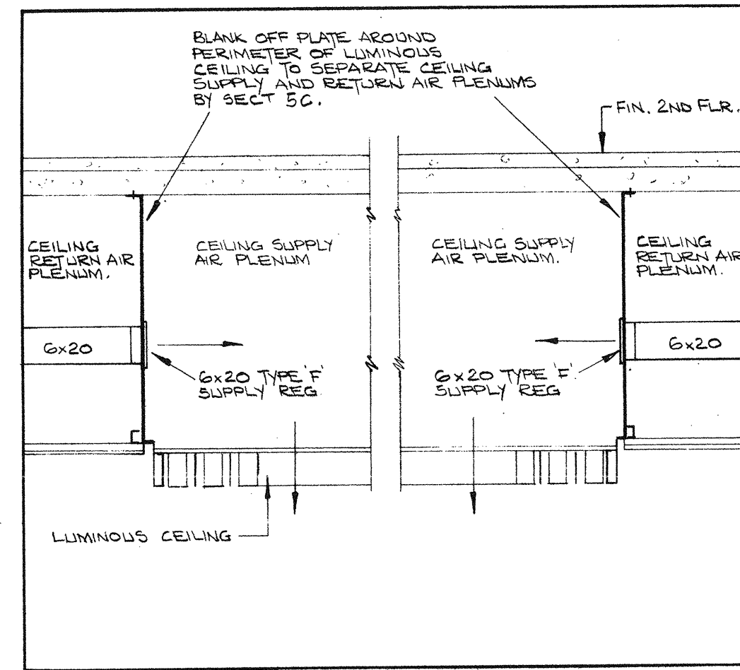
16 TYPICAL DETAIL OF AIR SUPPLY AT GROUND FLR. LUMINOUS CLG. SCALE: 1/2"=1'-0".
