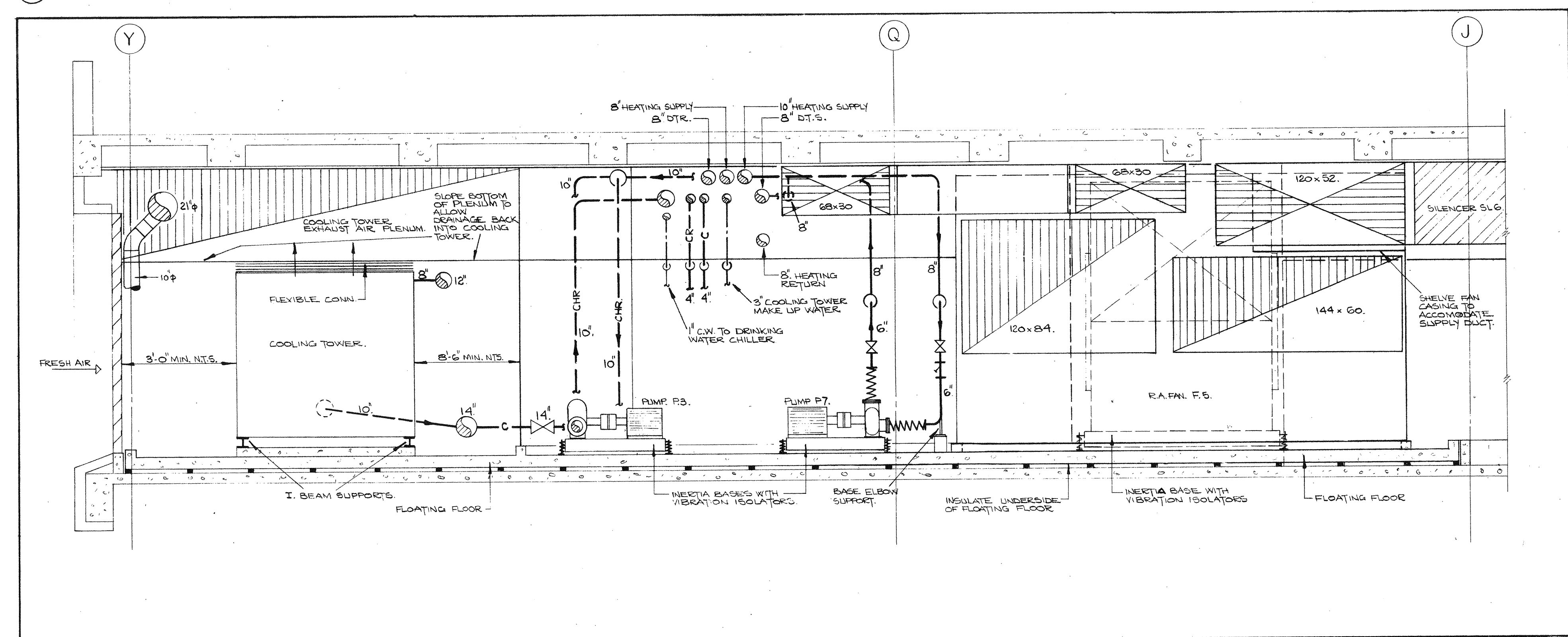
10 SECTION. SCALE: 1/4"=1'-0".
