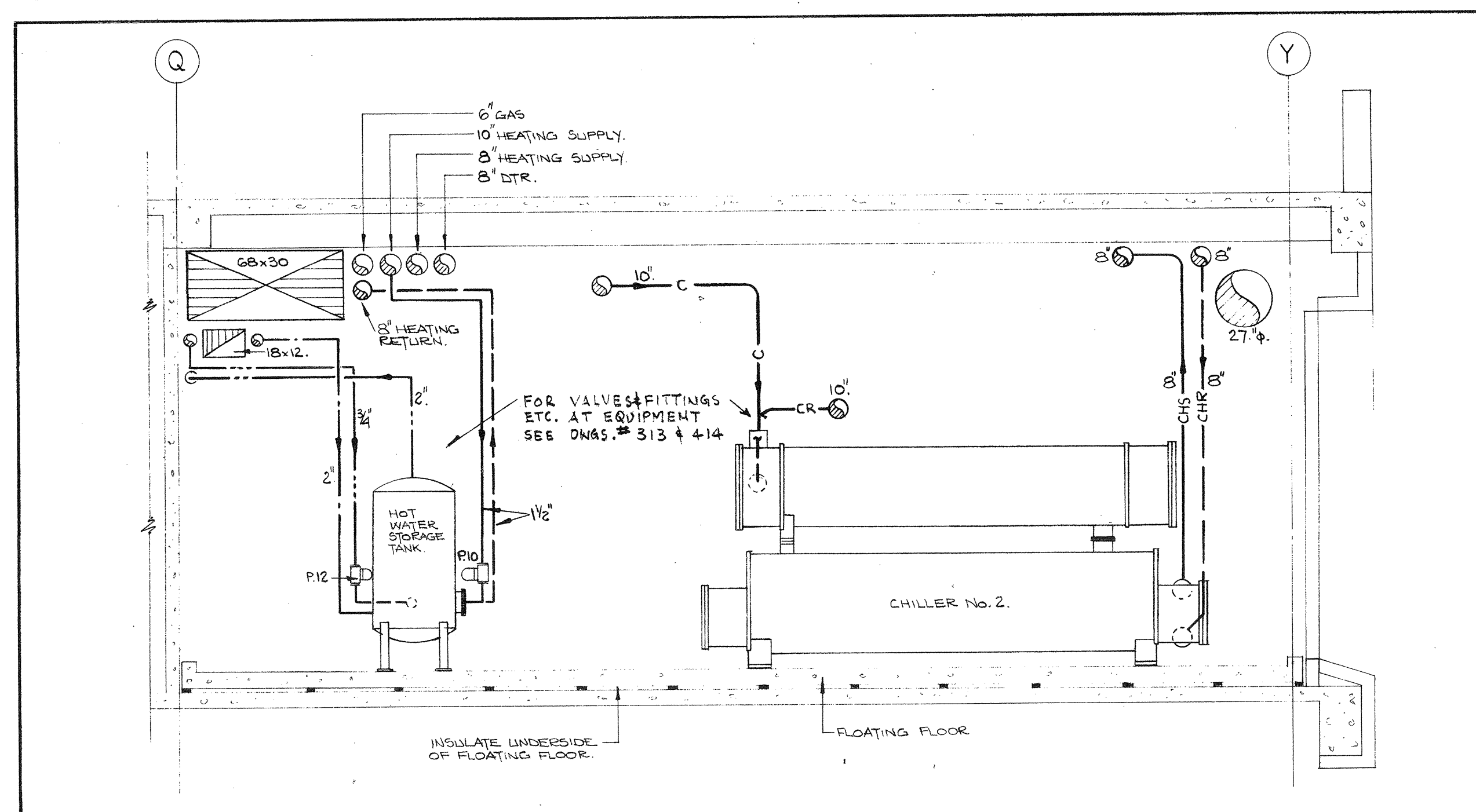
7 SECTION. SCALE: 1/4"=1'-0".
