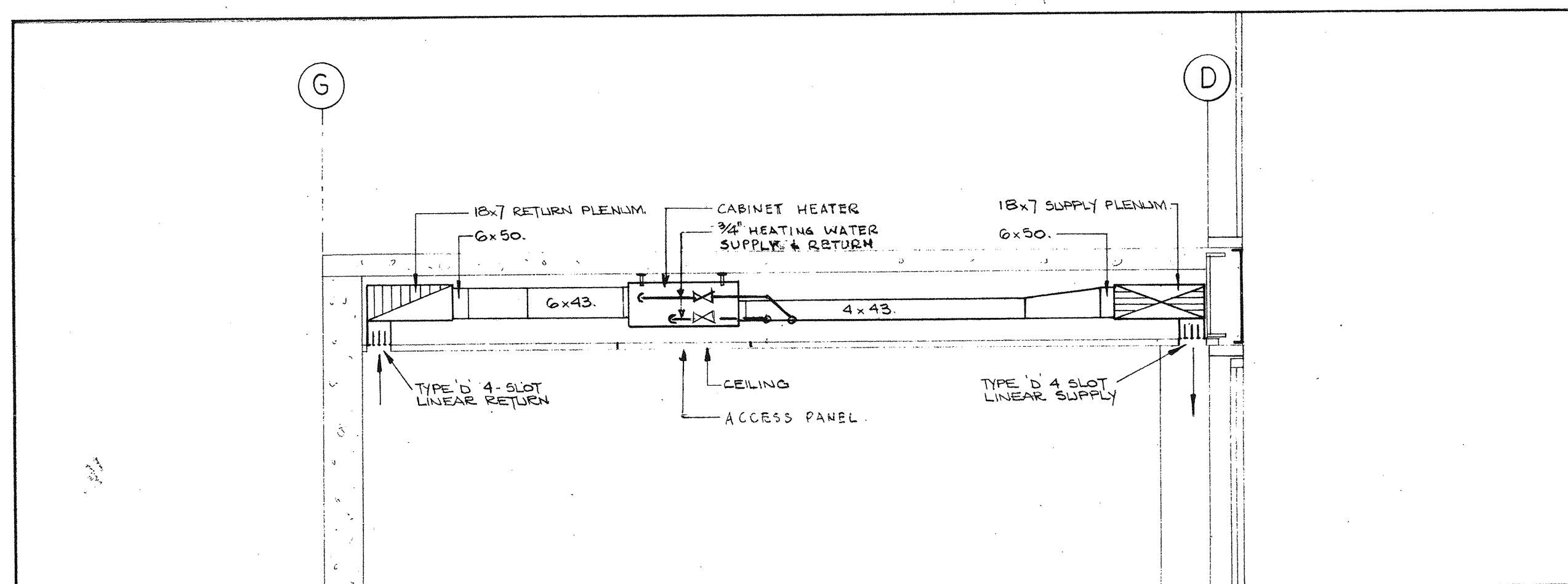
15 SECTION. STAIR No. 1. GROUND FLOOR. SCALE: 1/2"=1'-0".
