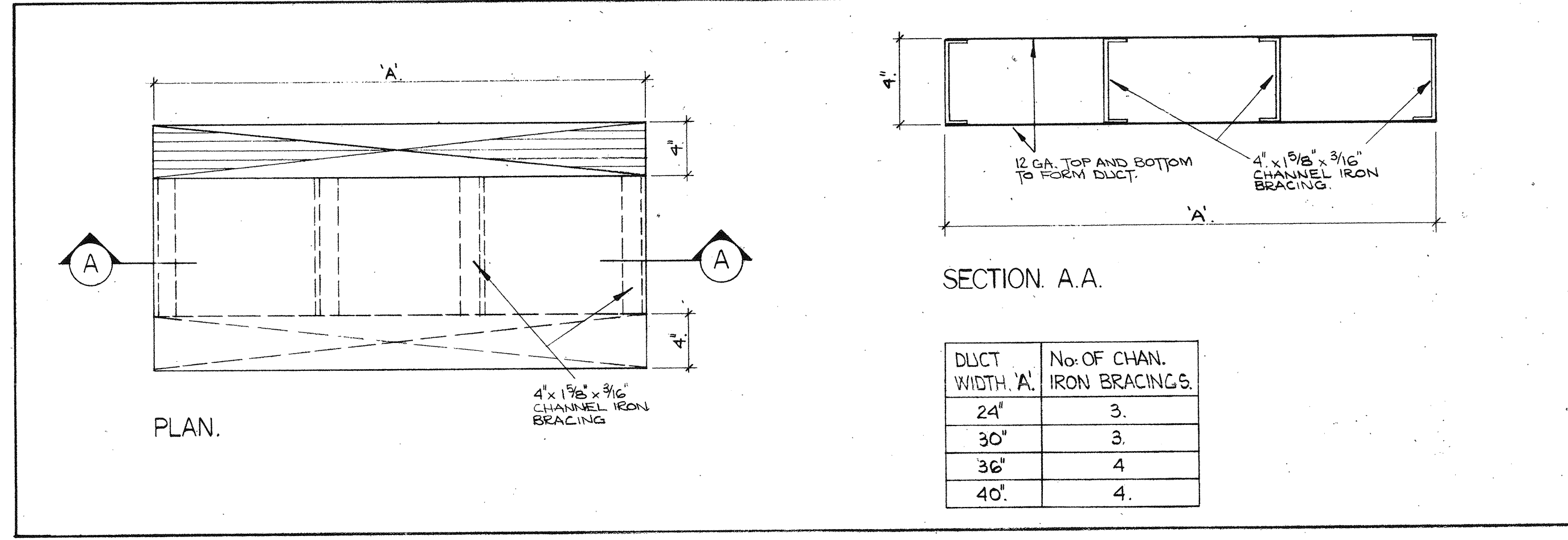
17 DETAIL OF BRACING REQUIRED FOR DUCTS POURED IN SLAB. N.T.S.
