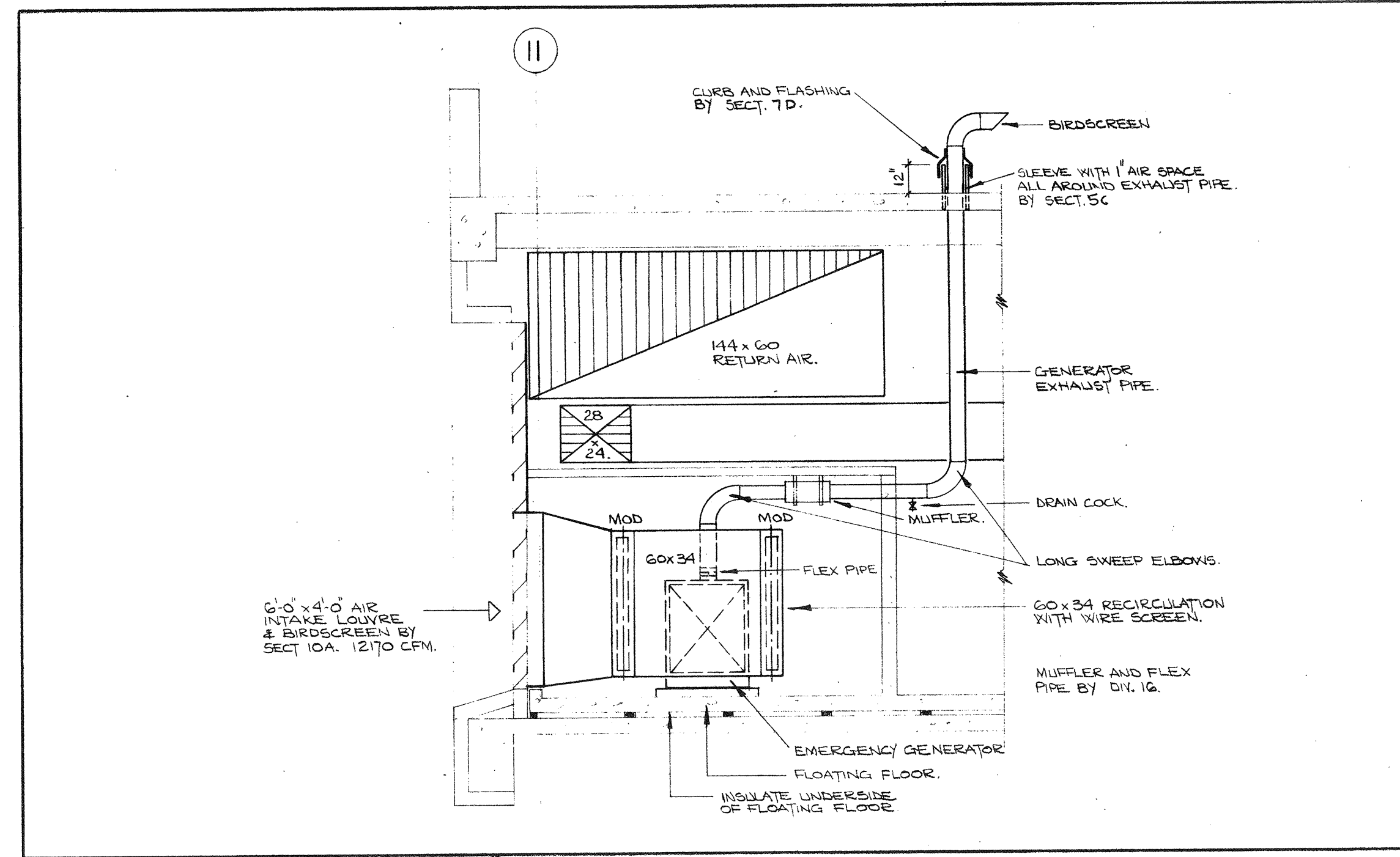
8 SECTION. SCALE: 1/4"=1'-0".
