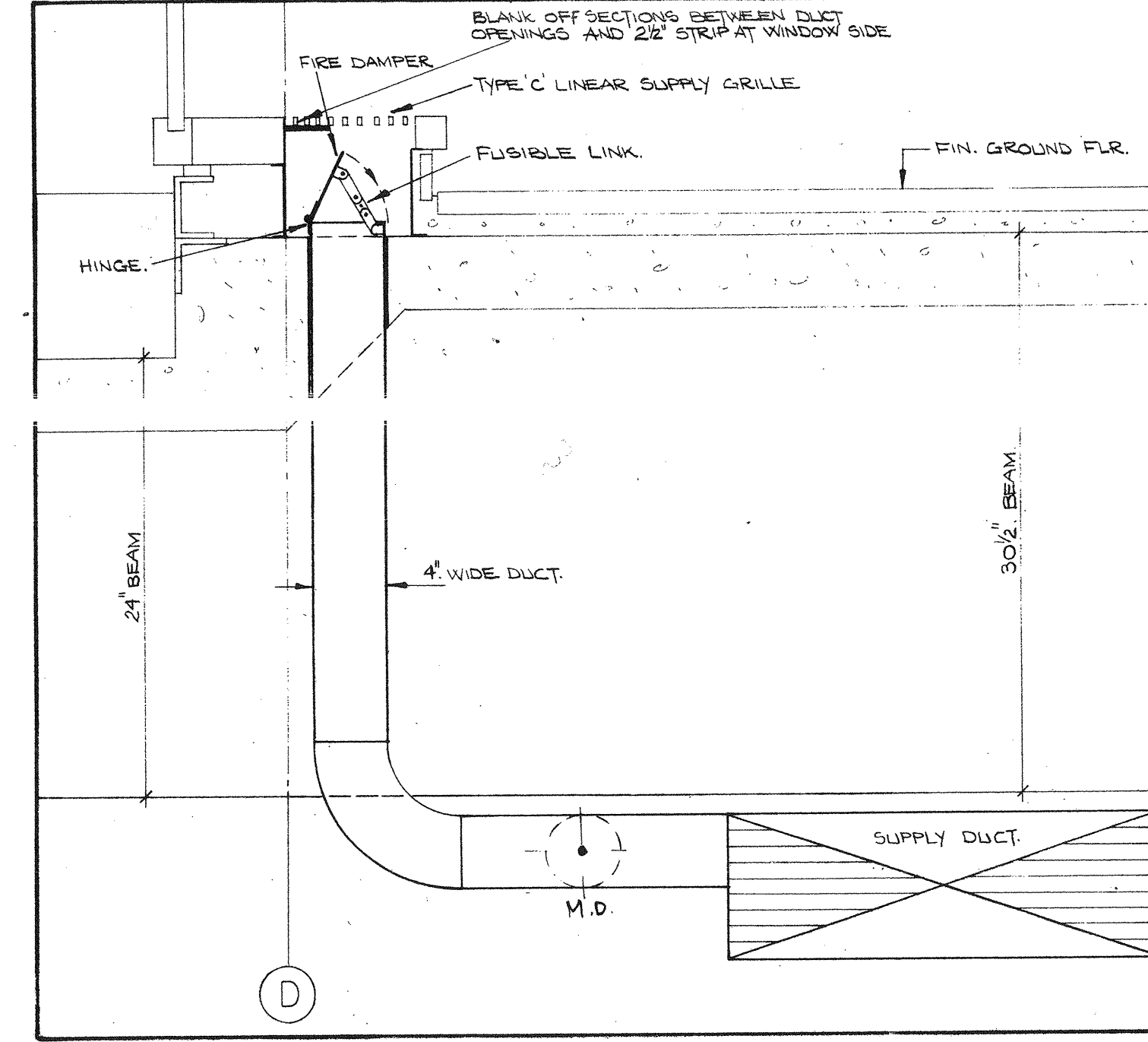
12 GROUND FLOOR WEST WINDOW SUPPLY DETAIL BETWEEN GRID LINES 10 & 33. SCALE: 1 1/2"=1'-0".
