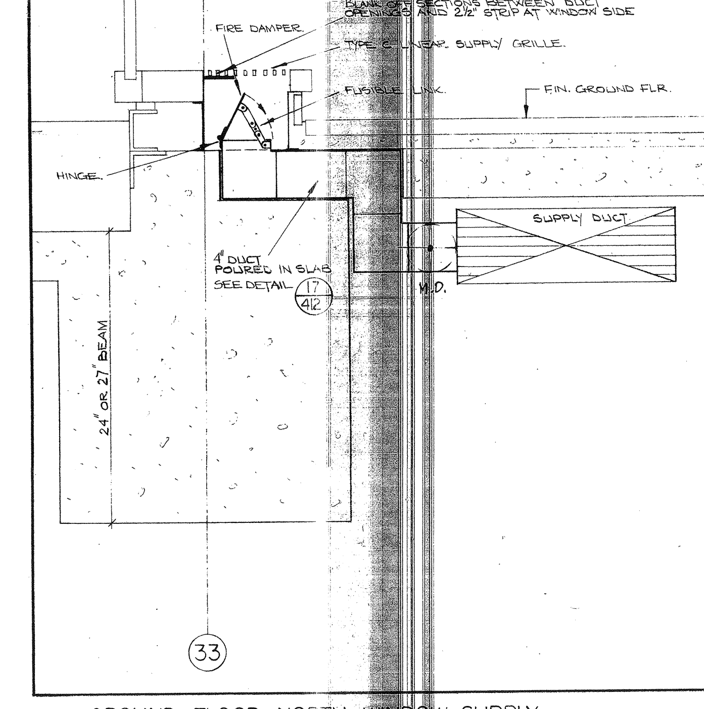
13 GROUND FLOOR NORTH WINDOW SUPPLY DETAIL BETWEEN GRID LINES D & V. SCALE: 1 1/2"=1'-0".
