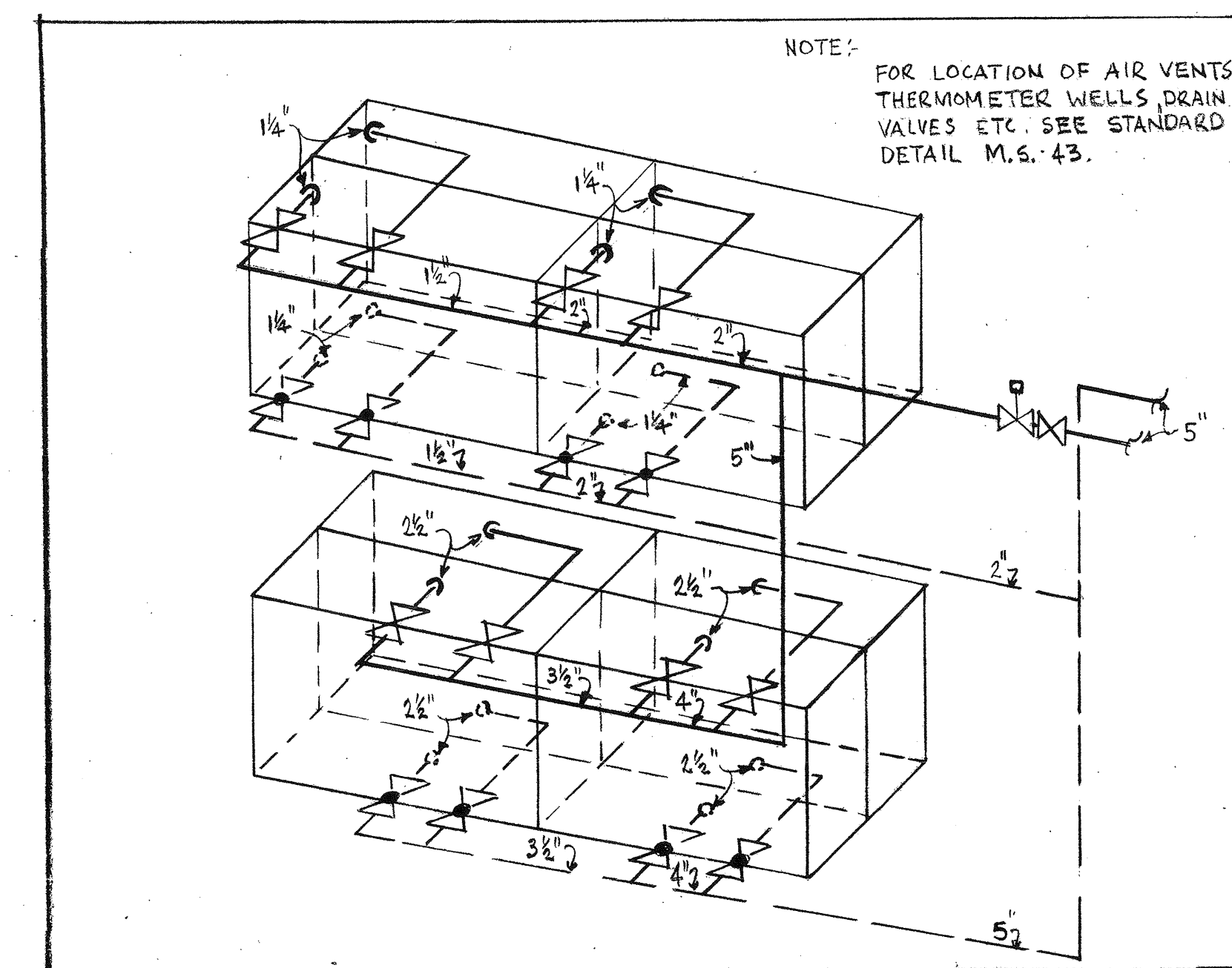
PIPING HOOK UP FOR GARAGE HEATING COILS.
