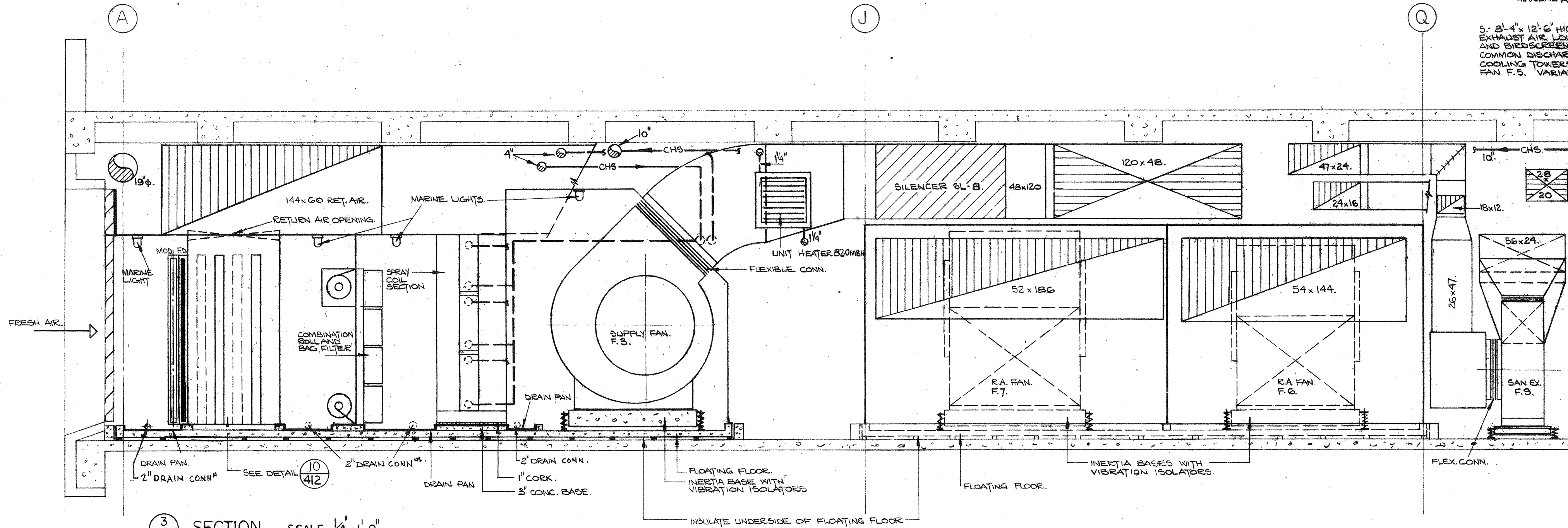
3 SECTION. SCALE: 1/4"=1'-0"
