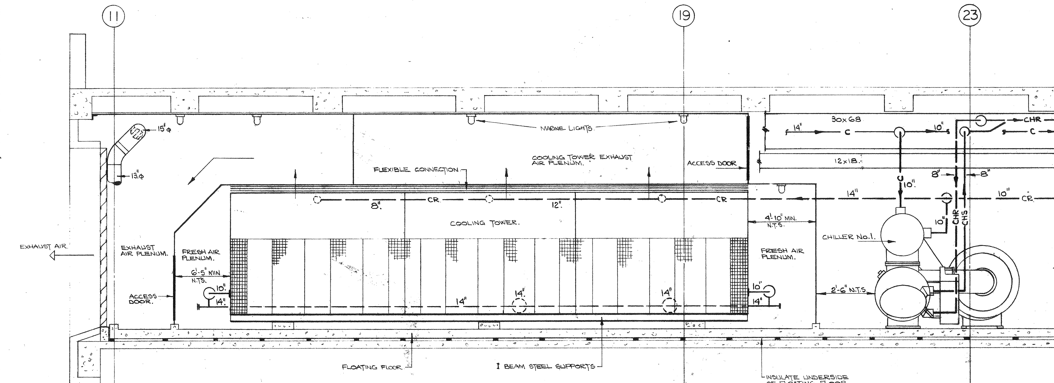
2 SECTION. SCALE: 1/4"=1'-0"
