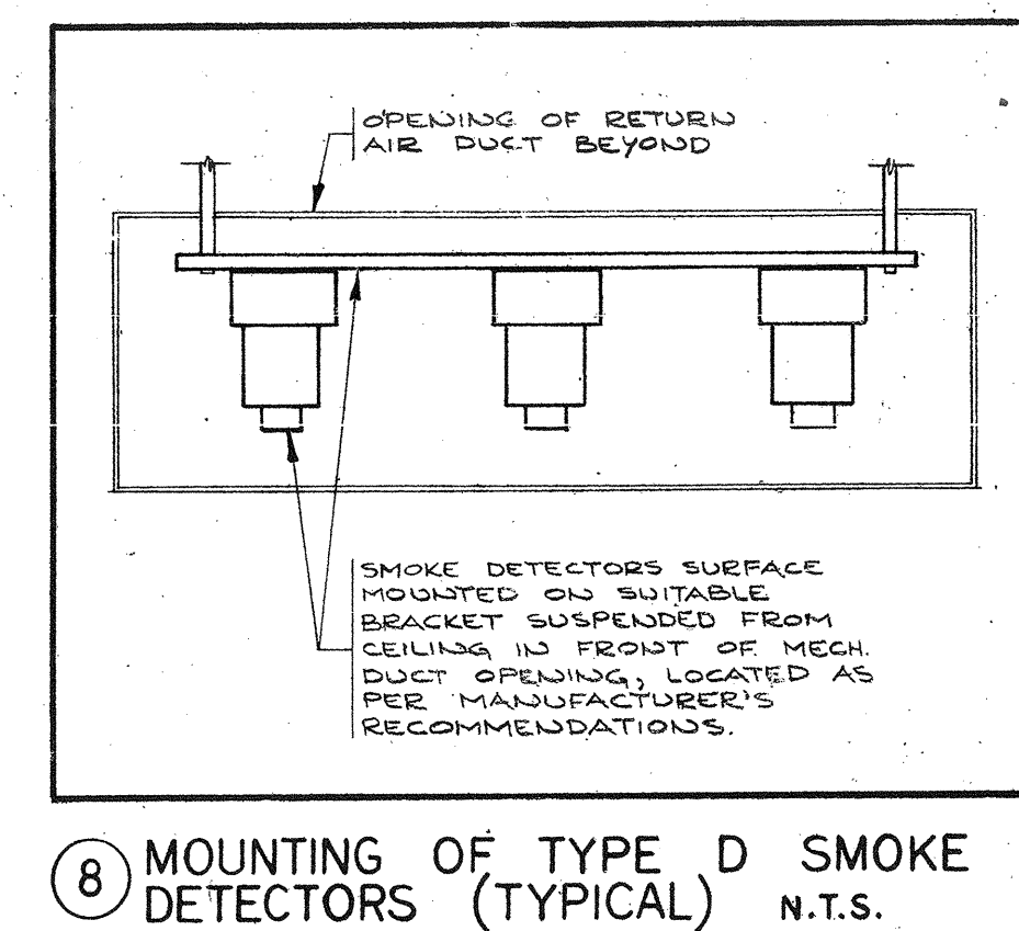
8 MOUNTING OF TYPE D SMOKE DETECTORS (TYPICAL) N.T.S.
