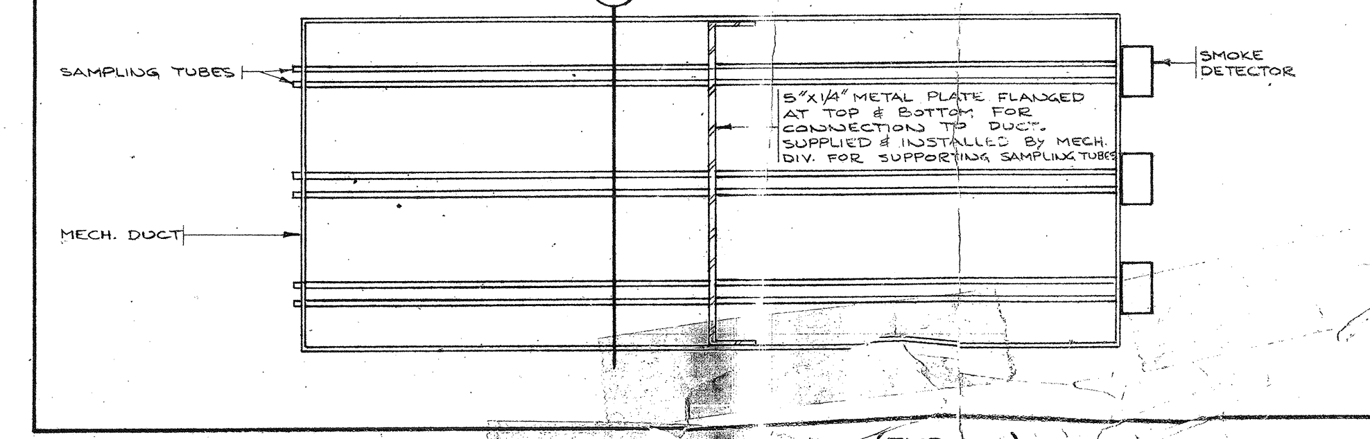
10 MOUNTING OF TYPE E SMOKE DETECTOR (TYPICAL) N.T.S.
