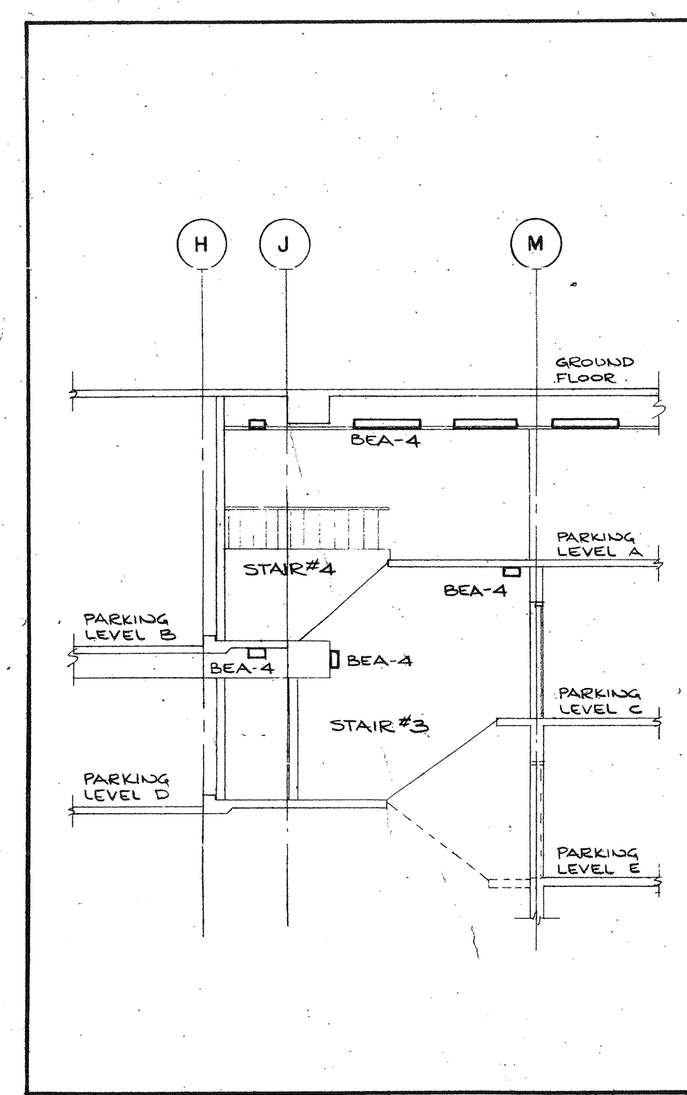
6 STAIRS S3 AND S4 LIGHTING RISER SCALE: 1/8"=1'-0"
