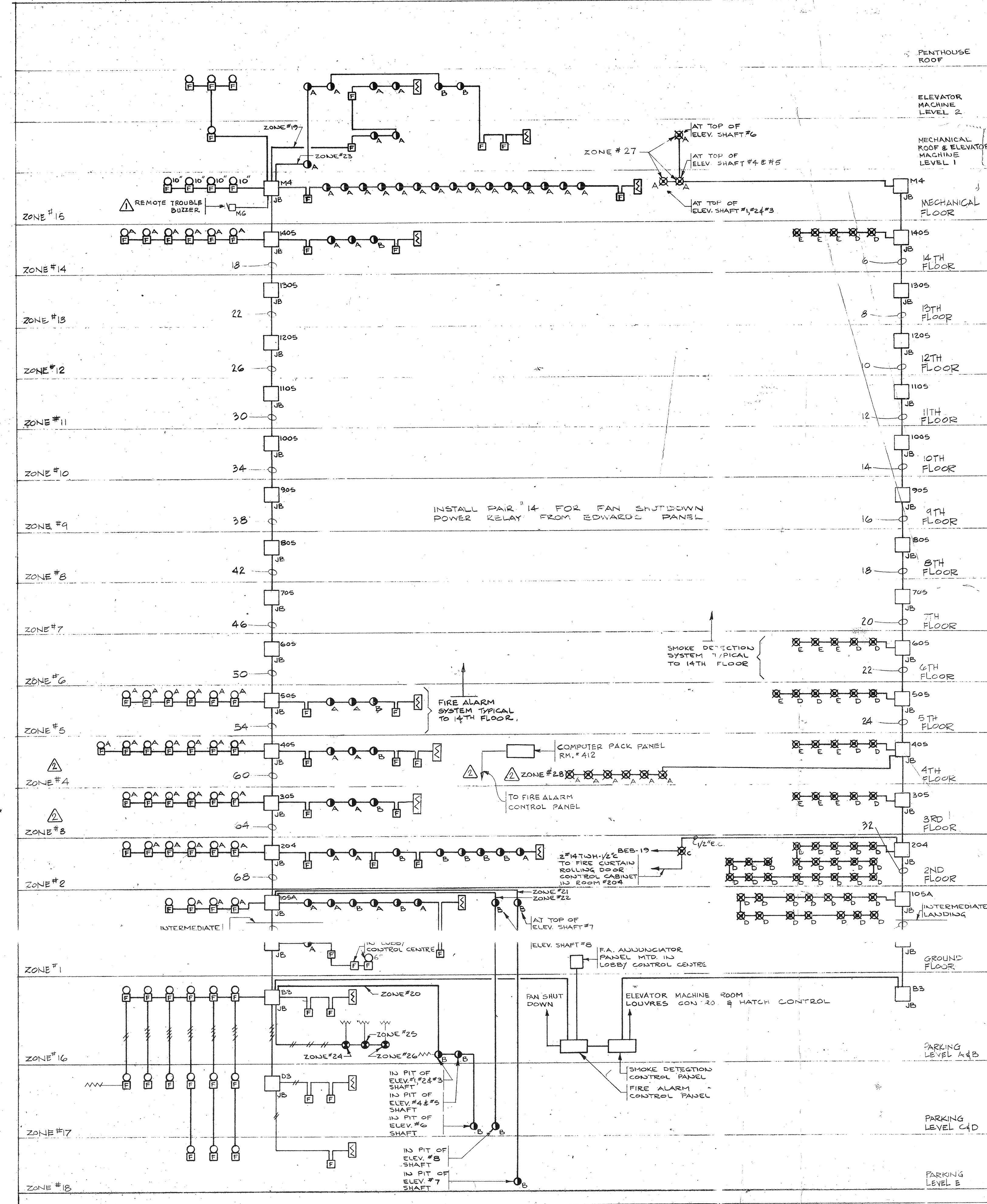
4 FIRE ALARM AND SMOKE DETECTION SYSTEMS RISER N.T.S.
