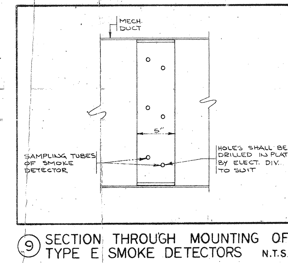
9 SECTION THROUGH MOUNTING OF TYPE E SMOKE DETECTORS (TYPICAL) N.T.S.
