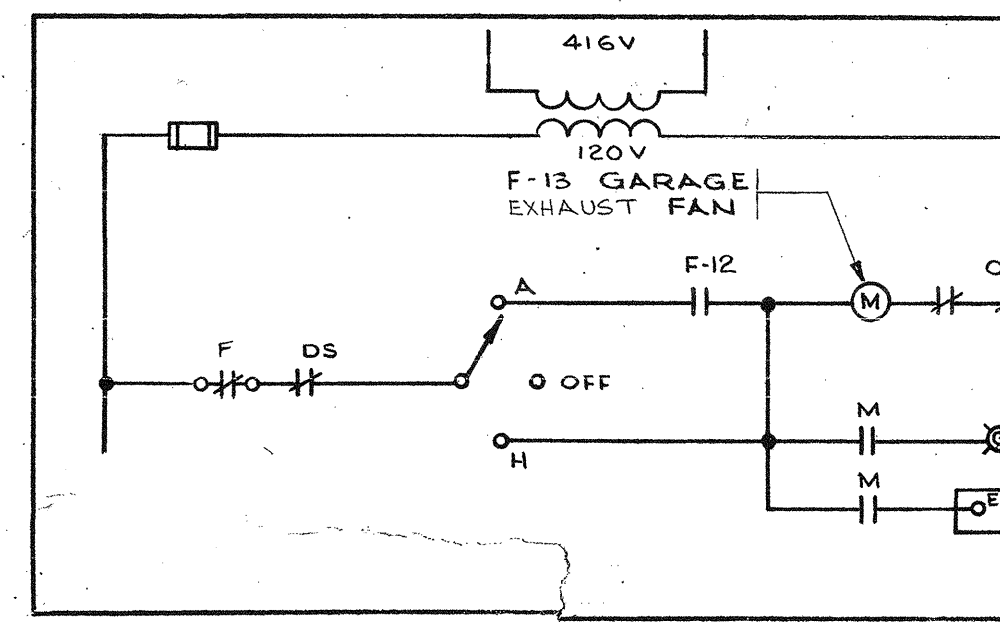
11 SCHEMATIC #10
