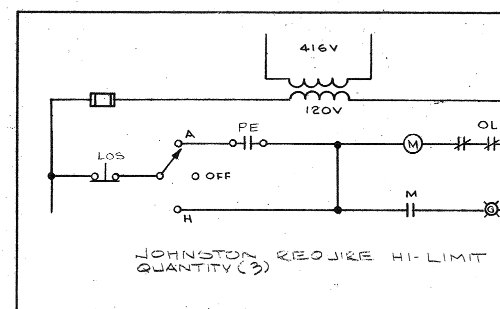
6 SCHEMATIC #5
