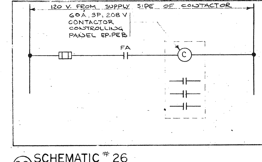
30 SCHEMATIC #29
