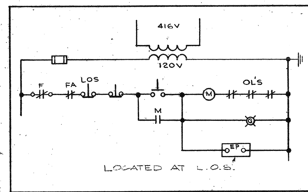
8 SCHEMATIC #7
