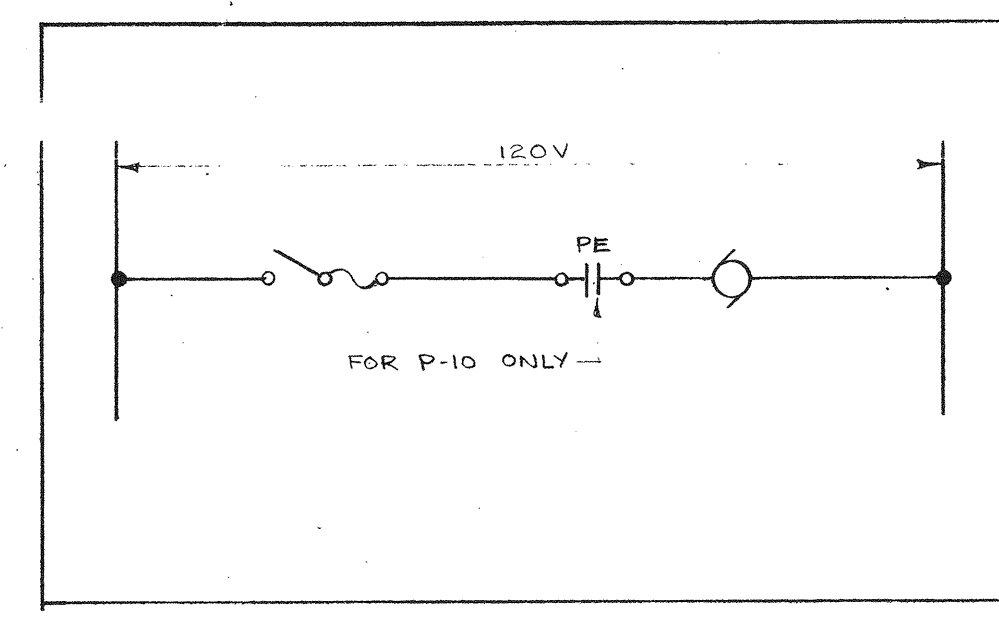
23 SCHEMATIC #21
