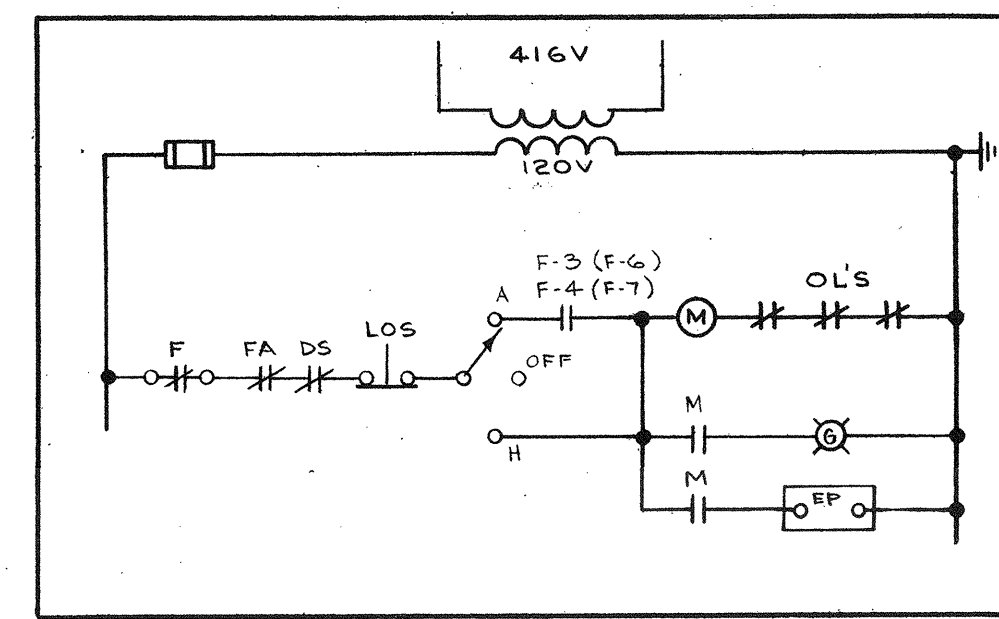
14 SCHEMATIC #13
