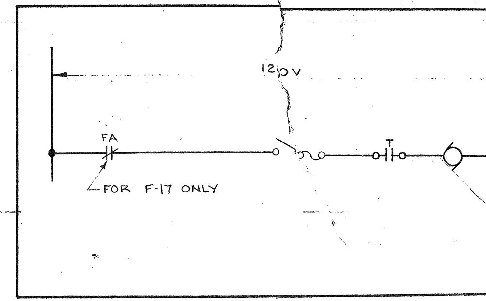
16 SCHEMATIC #15
