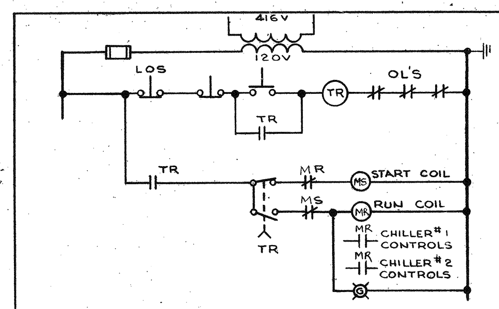
3 SCHEMATIC #2
