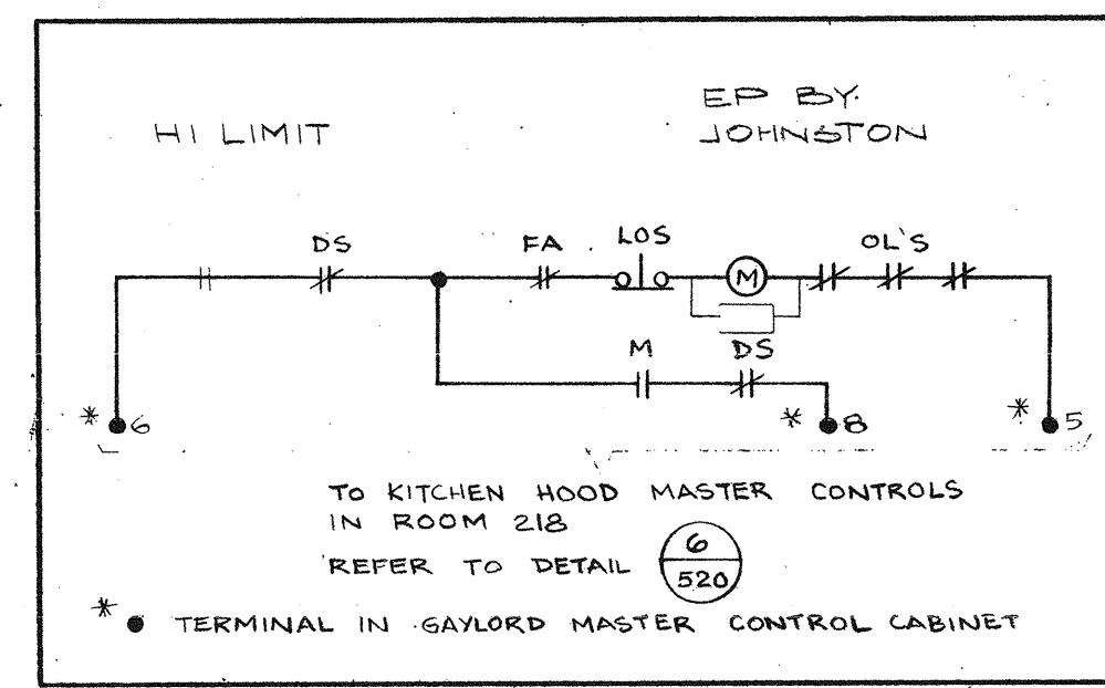
9 SCHEMATIC #8
