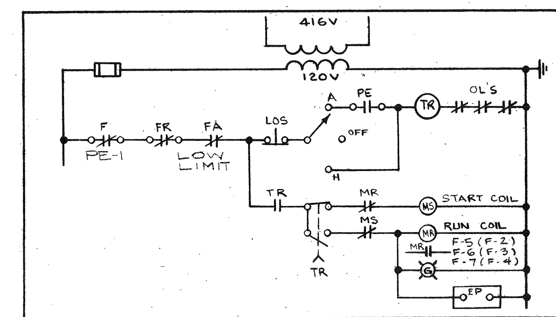
12 SCHEMATIC #11
