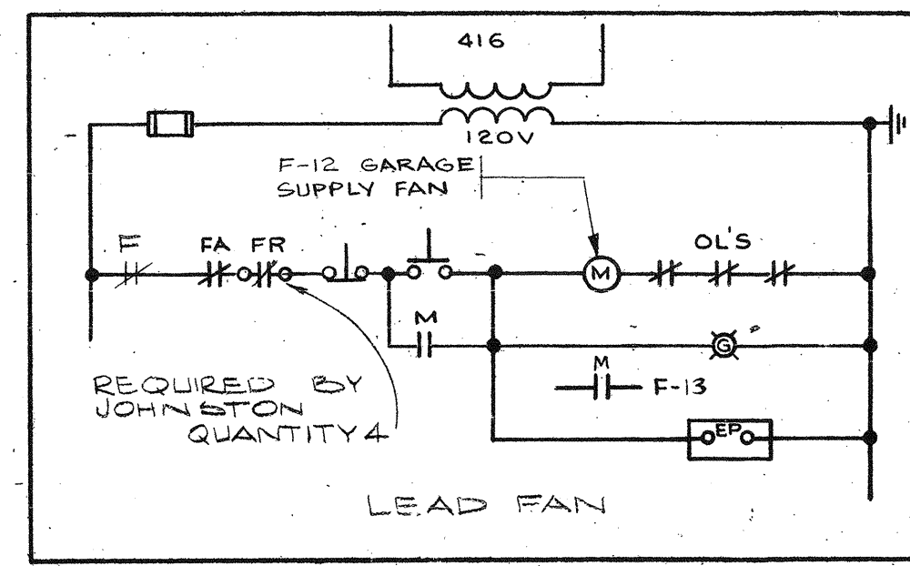
10 SCHEMATIC #9
