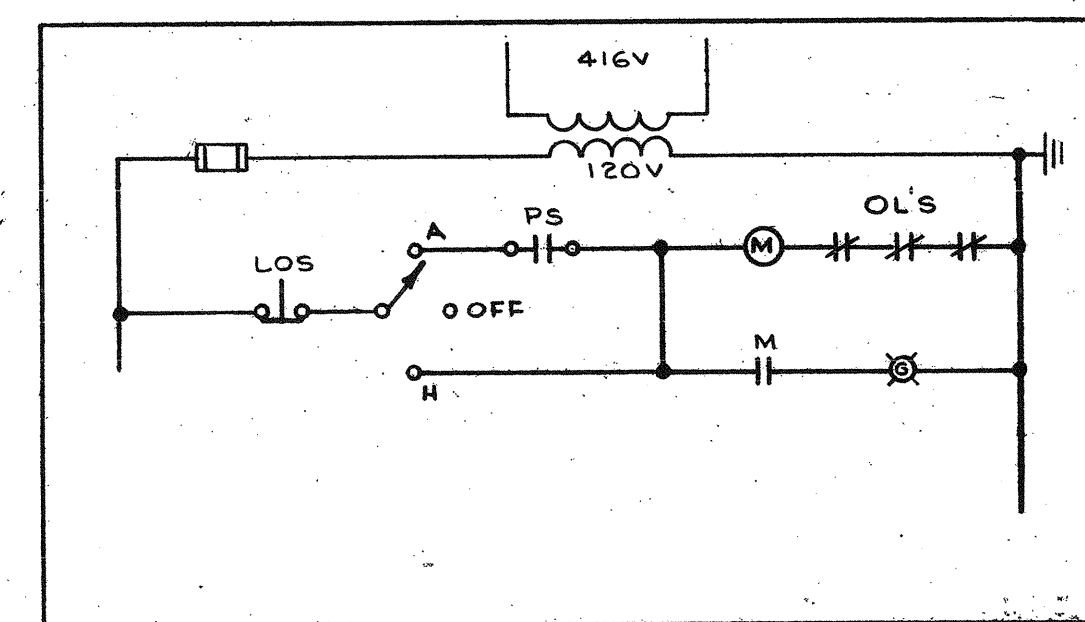
7 SCHEMATIC #6
