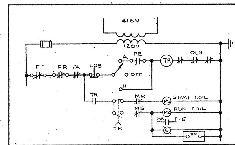
13 SCHEMATIC #12
