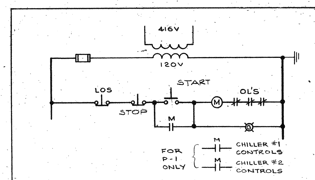
2 SCHEMATIC #1
