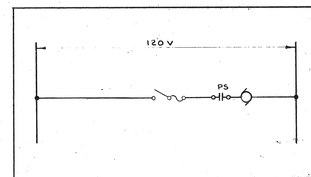
17 SCHEMATIC #16
