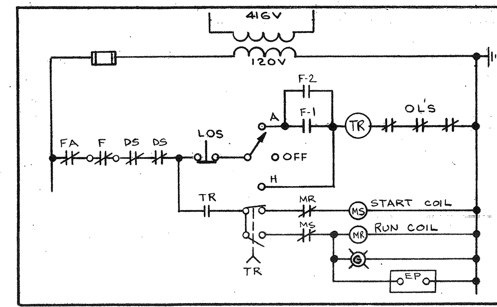
15 SCHEMATIC #14
