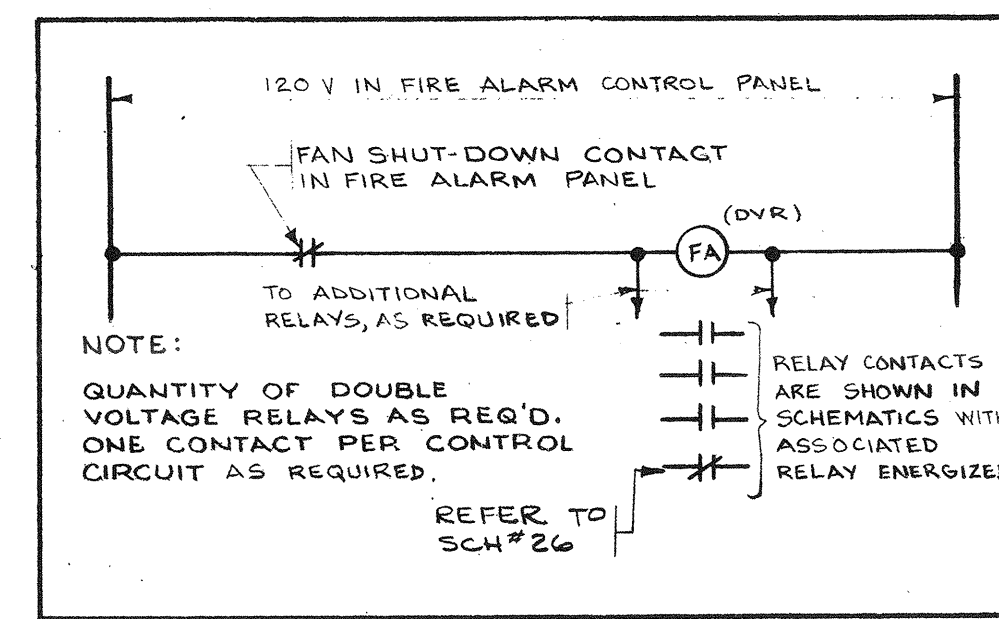
19 SCHEMATIC #18
