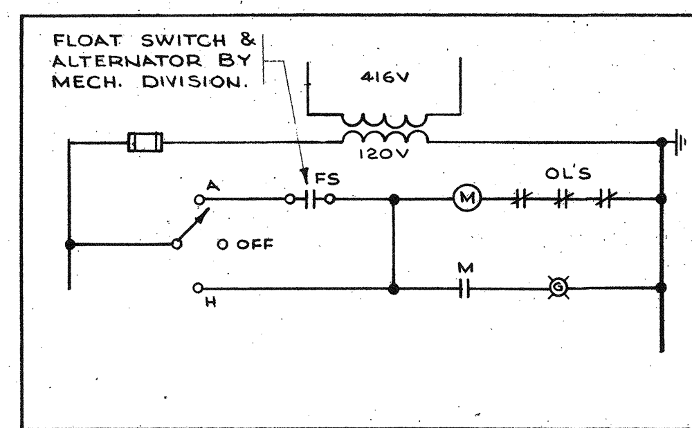
5 SCHEMATIC #4
