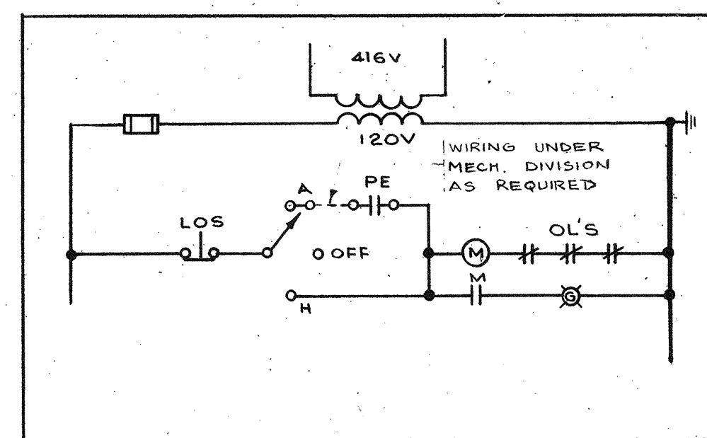
4 SCHEMATIC #3
