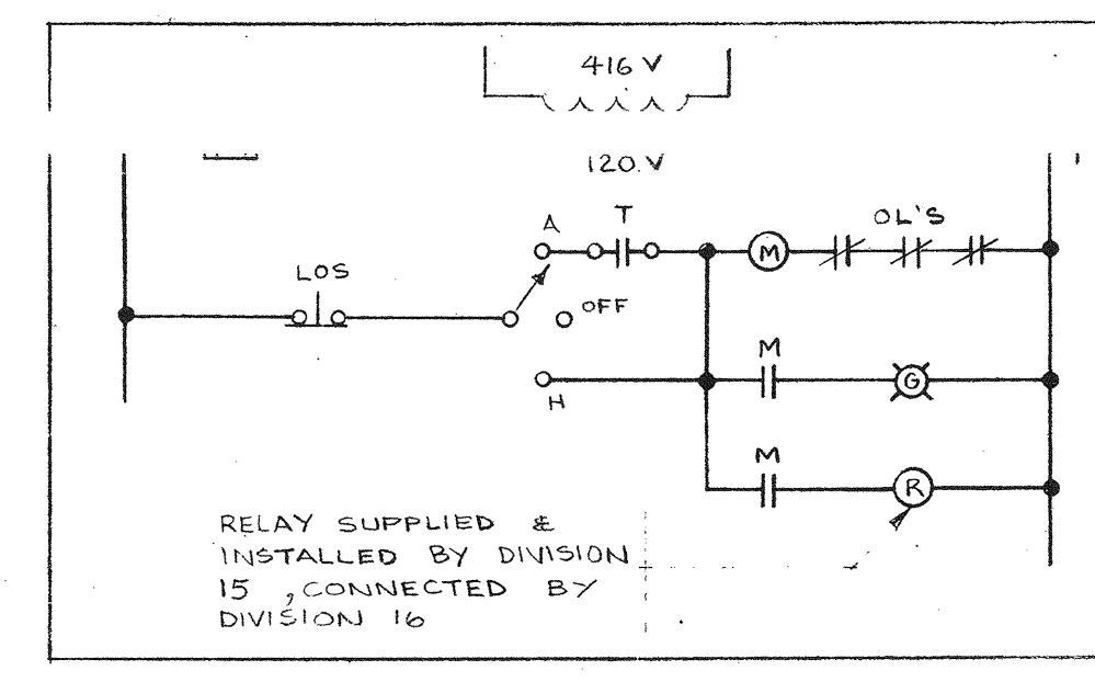
24 SCHEMATIC #22
