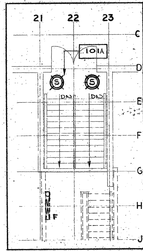
3 STAIR S1 LIGHTING AT INTERMEDIATE LANDING BETWEEN GROUND & 2ND FLOOR. SCALE 1/8"=1'-0"
