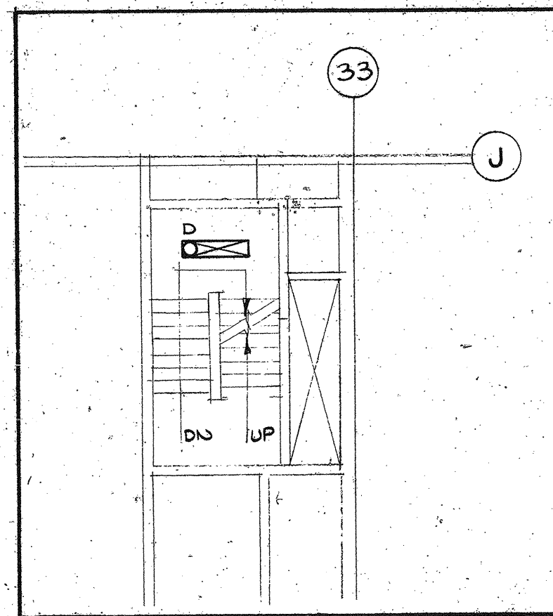
2 STAIR S5 LIGHTING AT INTERMEDIATE LANDING BETWEEN GROUND & 2ND FLOOR. SCALE 1/8"=1'-0"
