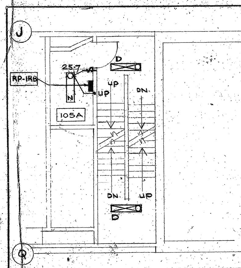
1 STAIR SI&S2 LIGHTING AT INTERMEDIATE LANDING BETWEEN GROUND & 2ND FLOOR. SCALE 1/8"=1'-0"
