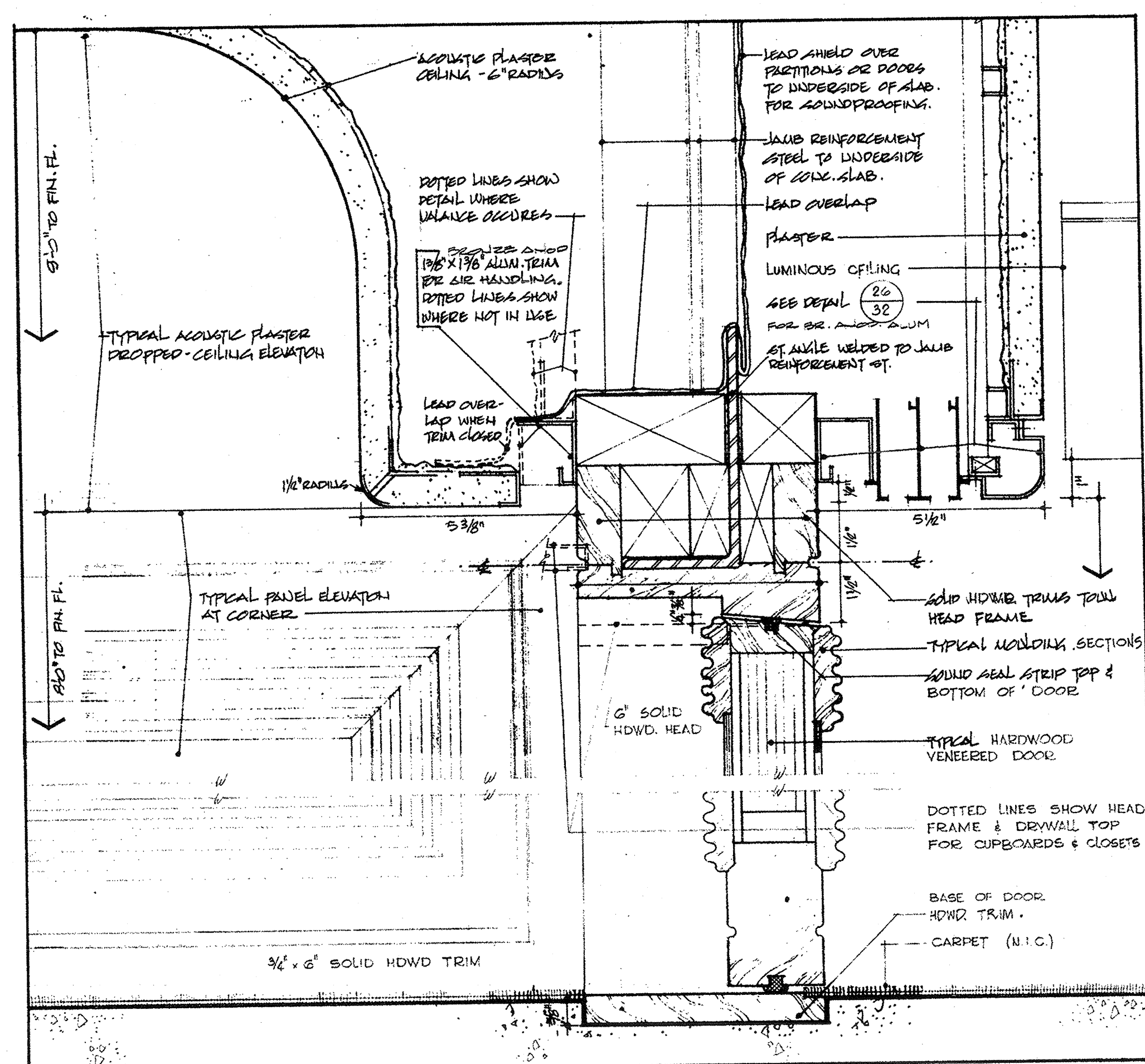
1/33 TYPICAL SECTION AT OFFICE DOOR & SECRETARIES AREA
