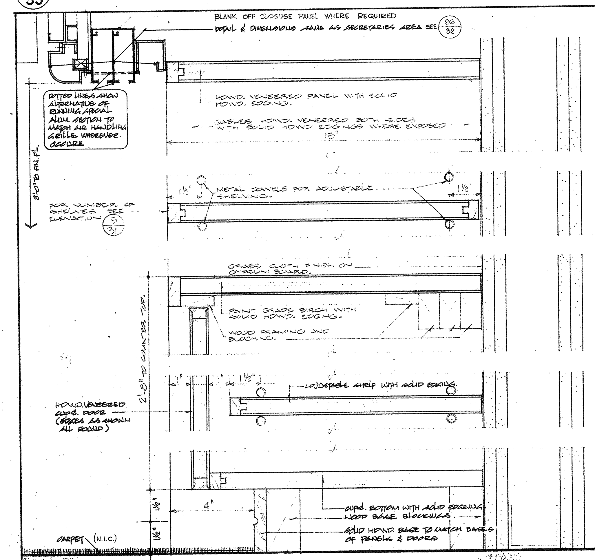
14/33 SECTION - CUPBOARD & SHELVING - OFFICE 518 & 519
