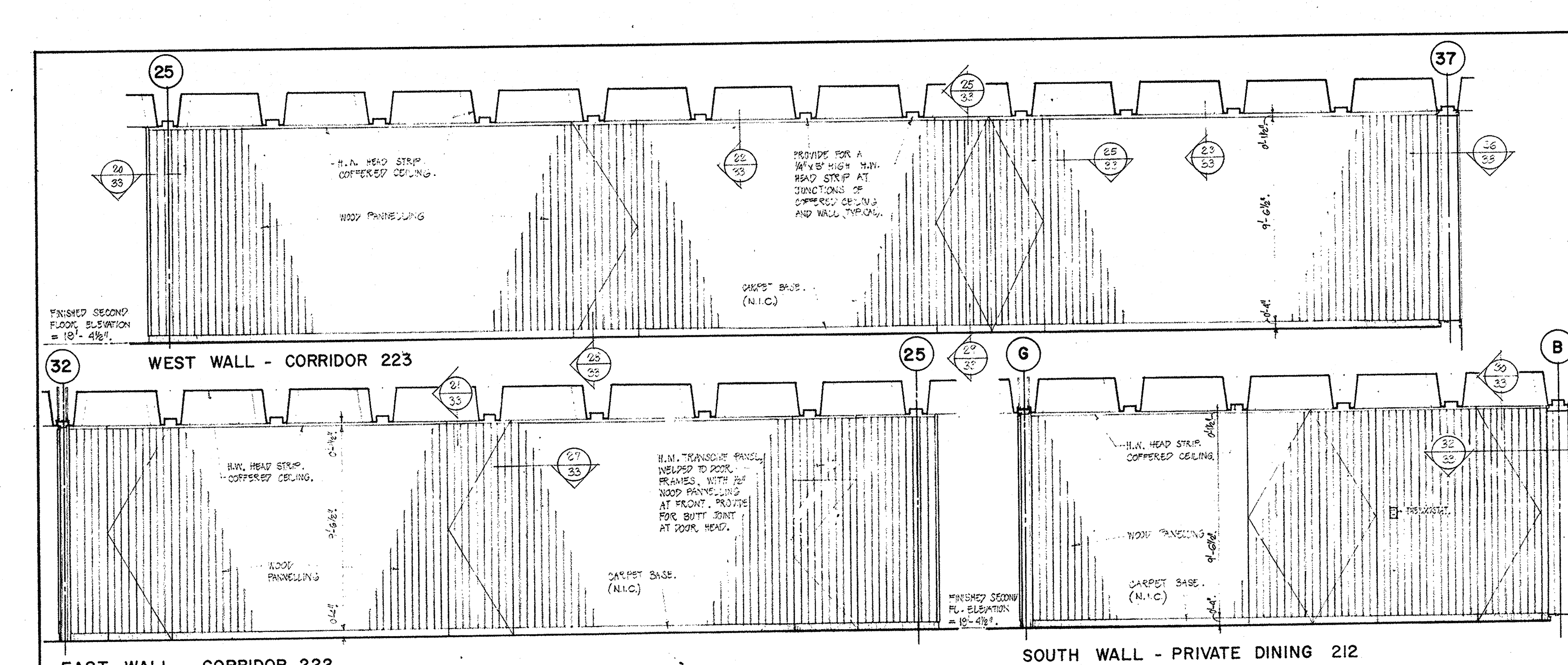
19/33 ELEVATION - WOOD PANELLED WALLS - SECOND FLOOR
