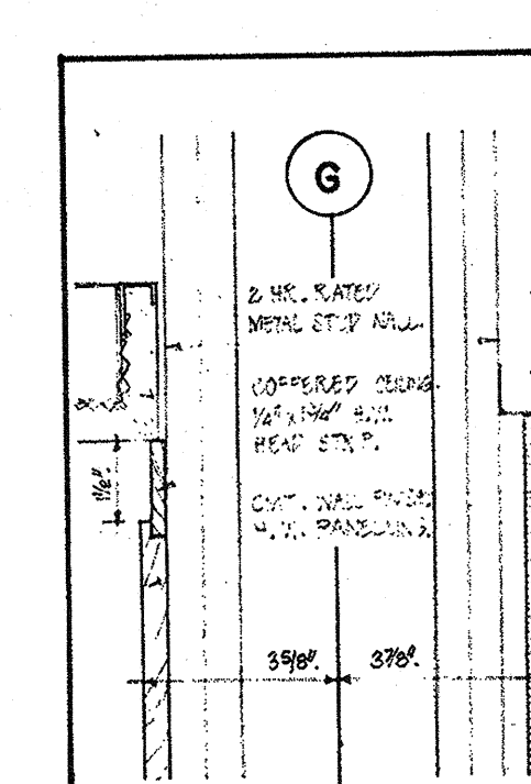
22/33 PARTITION HEAD
