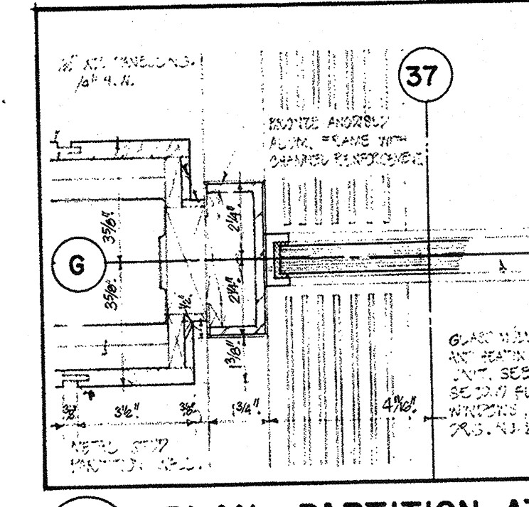
26/33 PLAN - PARTITION AT WINDOW WALL
