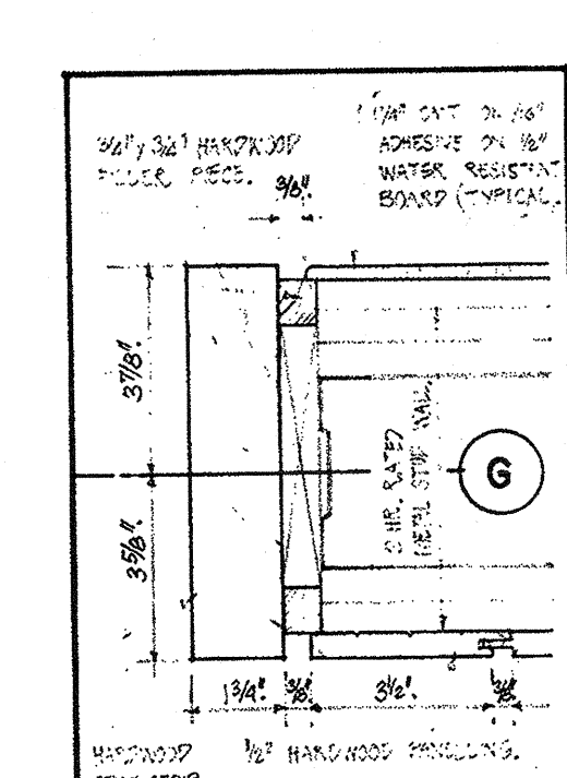
20/33 PLAN
