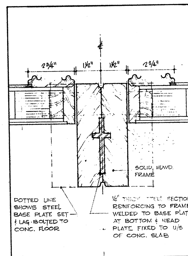
2/33 PLAN
