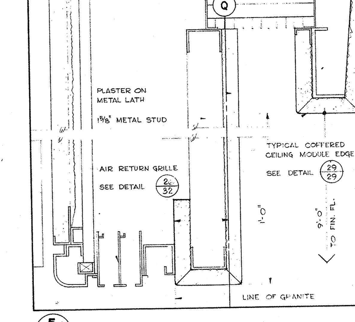
5/33 SECTION
