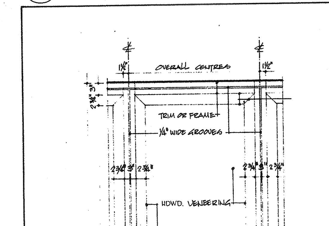
17/33 ELEVATION - TYPICAL DOOR OR FIXED PANEL
