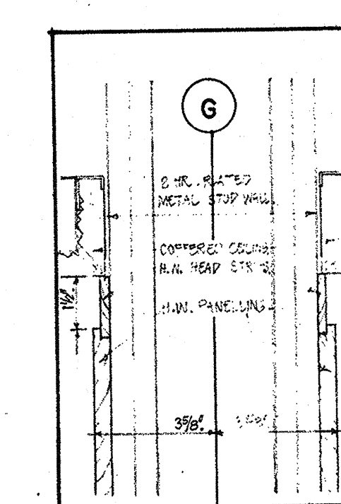
23/33 PARTITION HEAD
