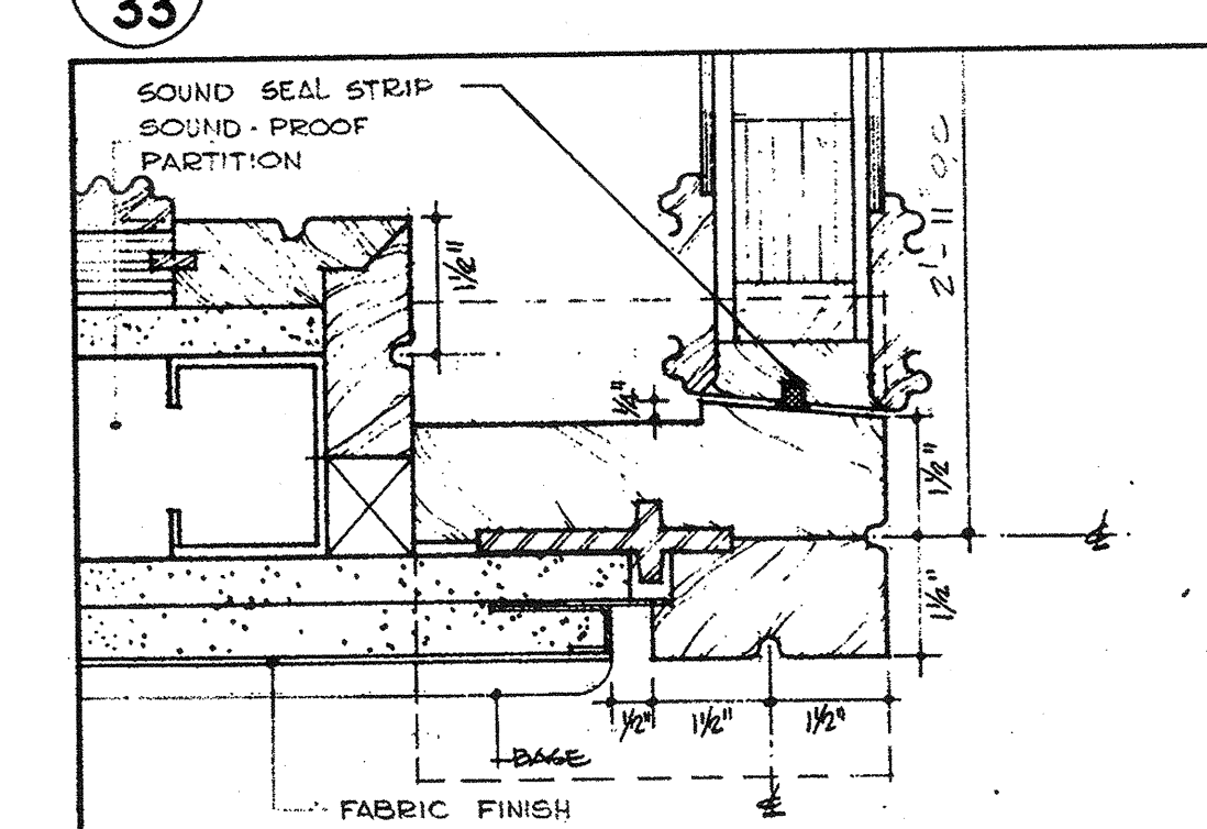
12/33 PLAN
