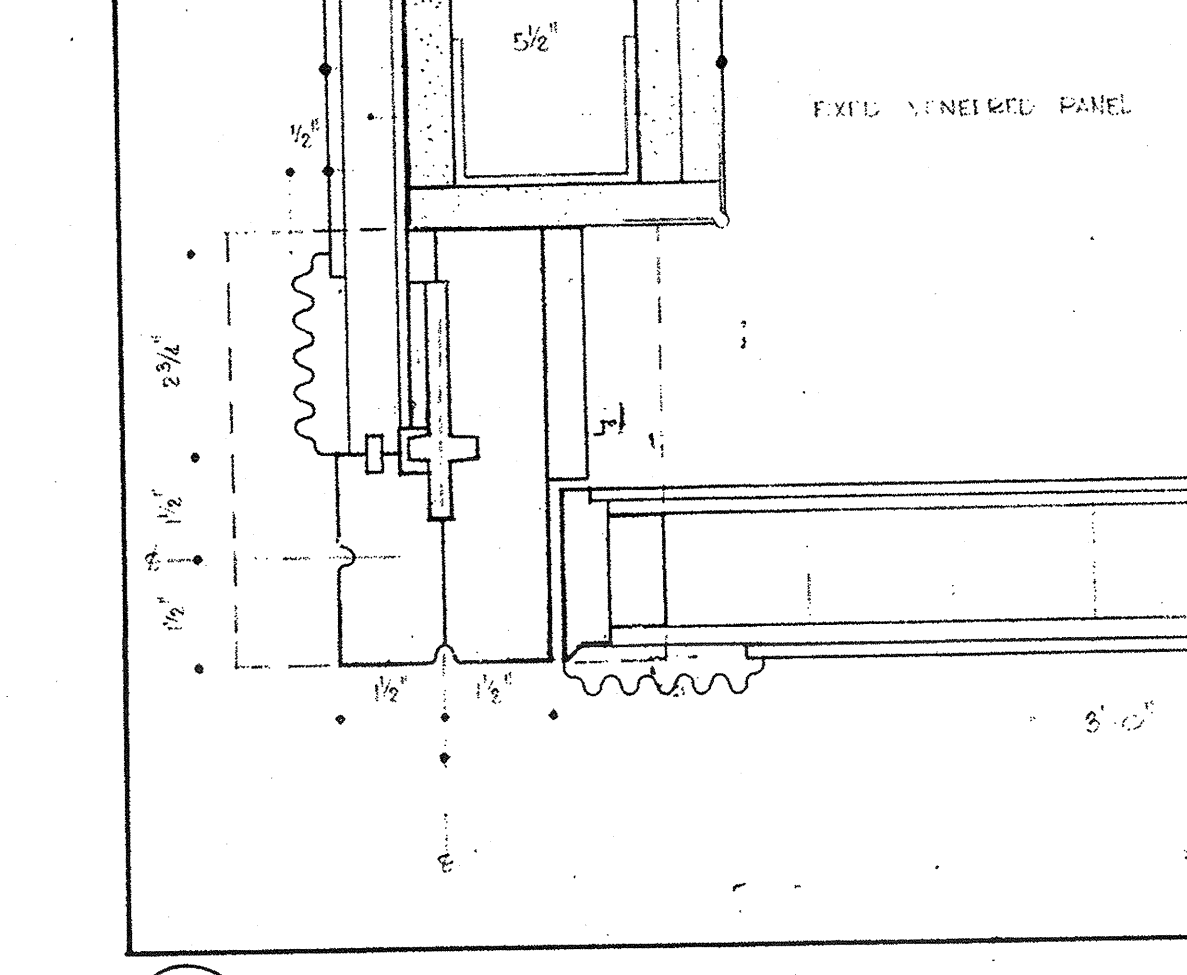
10/33 PLAN
