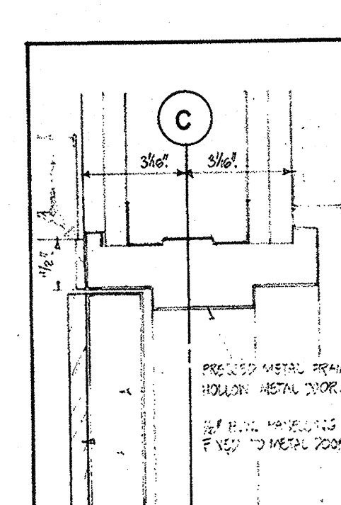
21/33 DOOR HEAD
