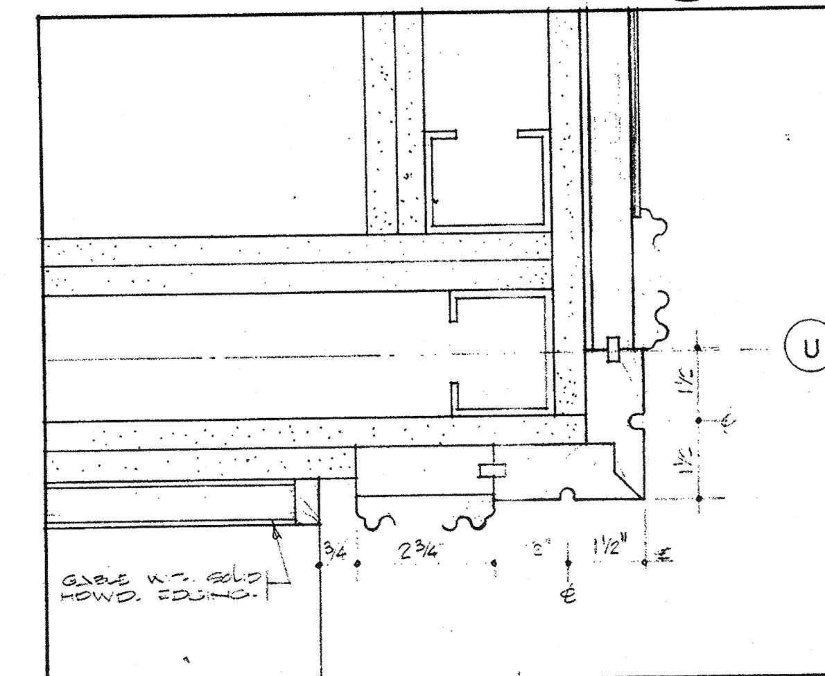
8/33 PLAN
