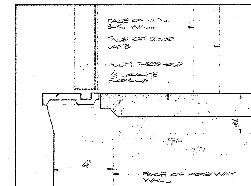
SECTION - THRESHOLD AT GROUND FL.
