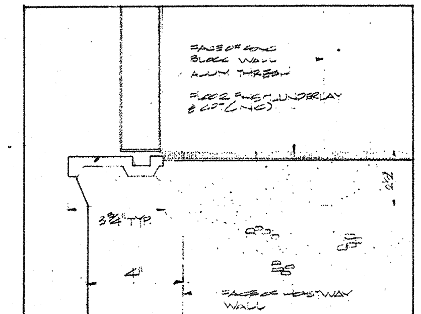
SECTION - THRESHOLD AT CARPET
