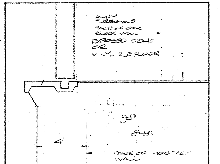
SECTION - TYP. THRESHOLD
