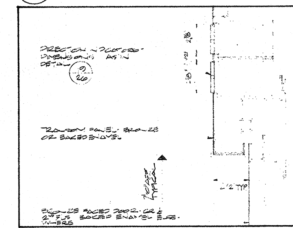
SECTION - TYP. TRANSOM PANEL AT ELEV. ENTRANCE
