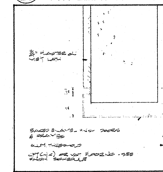
PLAN - JAMB AT TYP. ELEV. ENTRANCE
