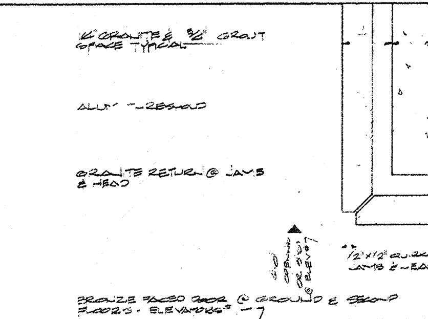
PLAN - JAMB AT GROUND, 2ND, 5TH FL. ELEV. ENTRANCE
