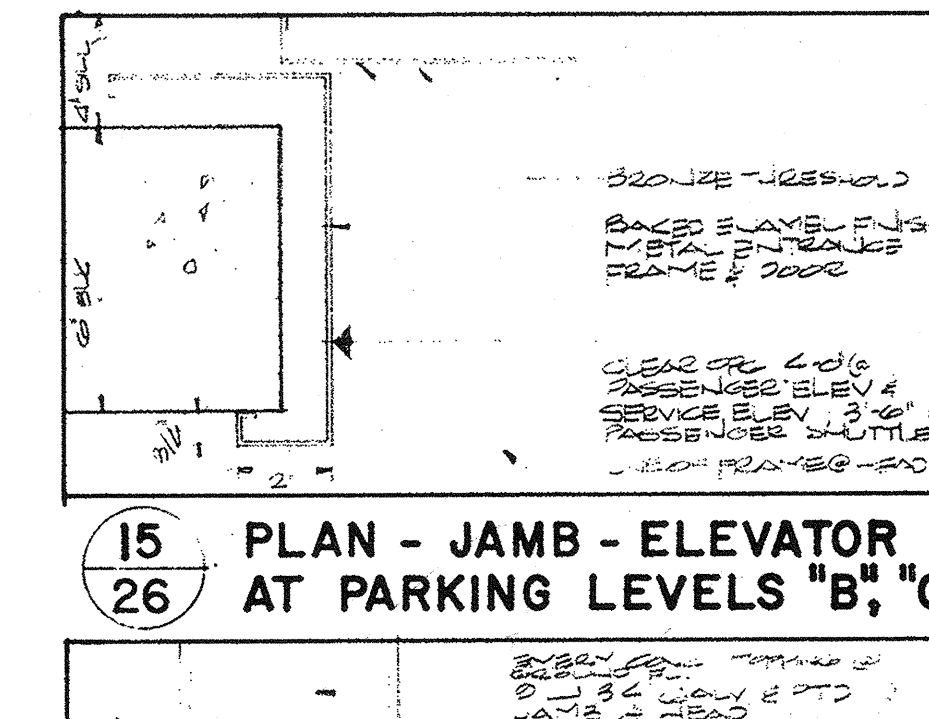
PLAN - JAMB - ELEVATOR AT PARKING LEVELS 'B', 'C', 'E'
